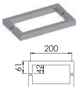
SQUARE PULL HANDLES
