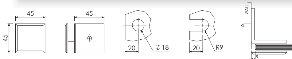
BEVEL 180° WALL TO GLASS CLAMP
