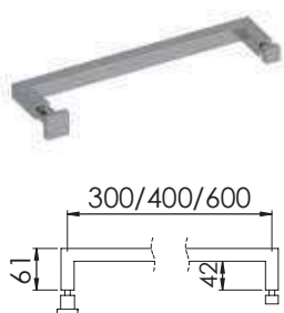
SQUARE TOWEL RAIL WITH BACK KNOB
