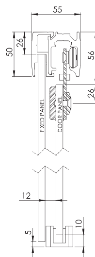
CLIP IN WHEEL WITH FIXED PANEL ADAPTER SECTION VIEW
