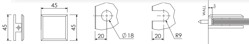
BEVEL 90° (L-CLAMP) WALL TO GLASS CLAMP
