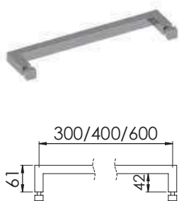
SQUARE TOWEL RAIL WITH FINIALS
