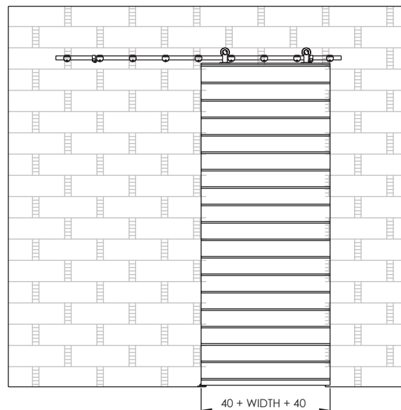
ELEVATION - WOOD SLIDER SIDE FIXED
