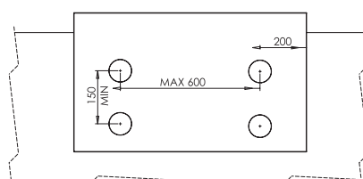
RECOMMENDED DETAILS
