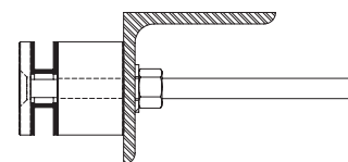
BEAM MOUNTED
