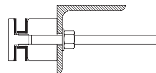
BEAM MOUNTED
