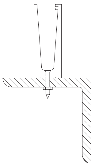
BEAM MOUNTED
