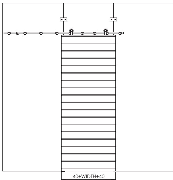
ELEVATION - WOOD SLIDER SHOPFRONT
