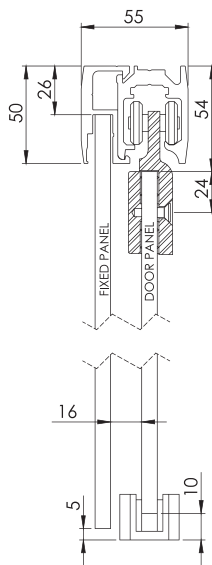
HEAVY DUTY WHEEL WITH FIXED PANEL ADAPTER SECTION VIEW
