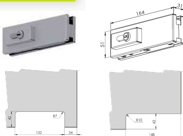
OPTION 1: CUTOUT OFFSET
