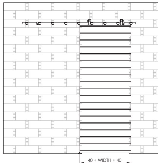
ELEVATION - WOOD SLIDER SIDE FIXED
