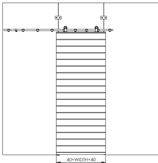
ELEVATION - WOOD SLIDER SHOPFRONT
