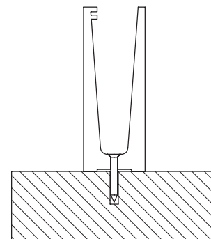
FLOOR MOUNTED
