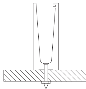
TIMBER MOUNTED
