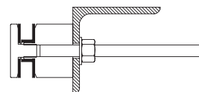
BEAM MOUNTED
