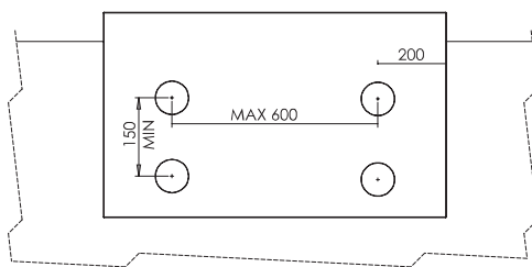
RECOMMENDED DETAILS
