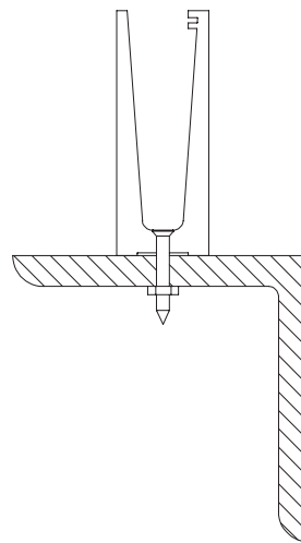
BEAM MOUNTED
