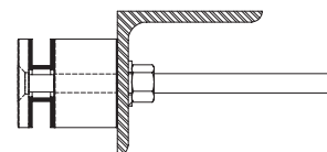
BEAM MOUNTED
